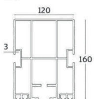
1 Rafter Profile
