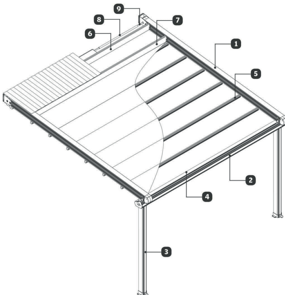
2 Gutter Profile
