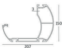
2 Gutter Profile
